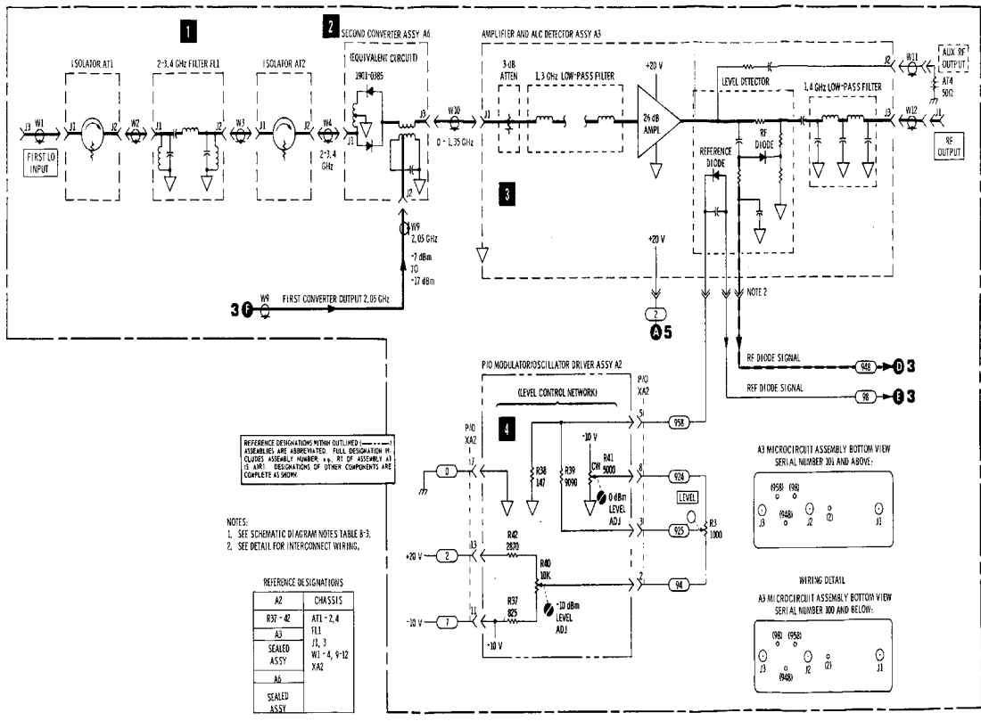
Figure 8-15. Second Converter Circuit, Schematic Diagram
