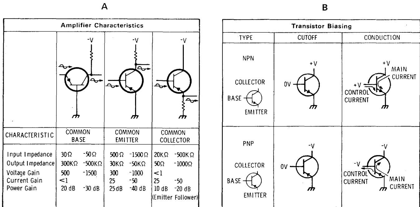
Figure 8-1. Transistor Operation 8-5
