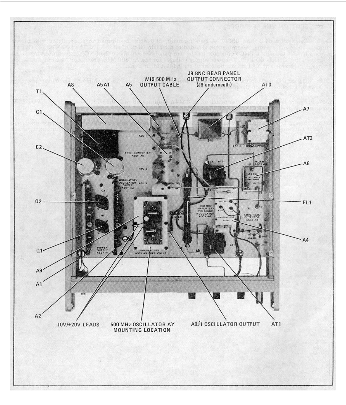
Figure D-1. 500 MHz LO Mounting location and Output Port for the 8444A, Option 058
