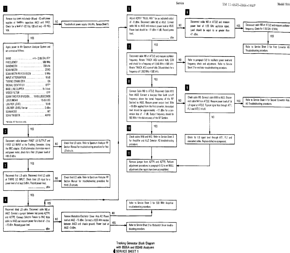
Figure 8-7A. Troubleshooting Tree
