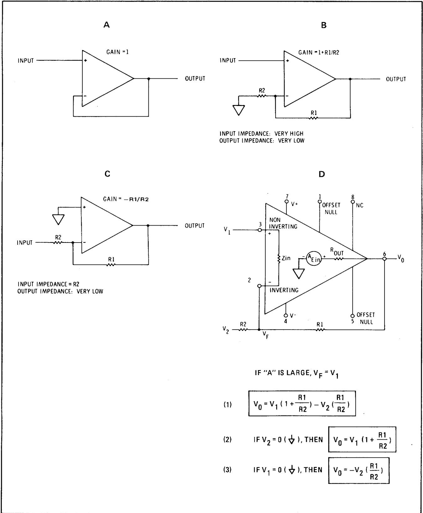
Figure 8-3. Operational Amplifier Equivalent Circuit 8-7/8-8
